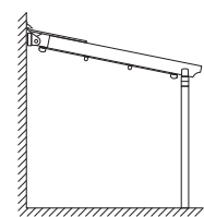
PITCHED MAX DIMENSIONS
